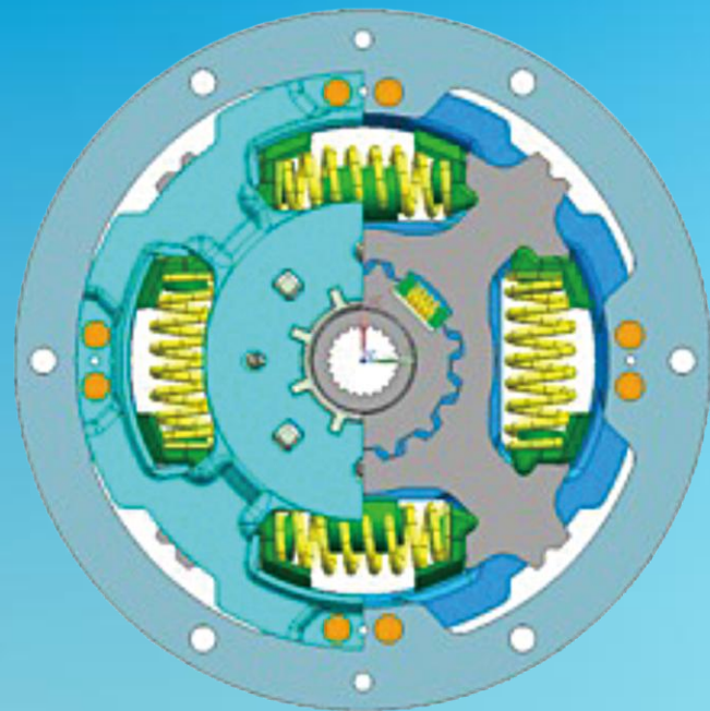
Conventional Damper
