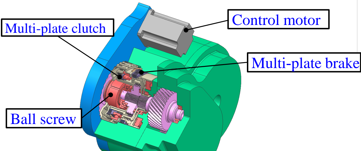
Unipres 2 speed transmission
